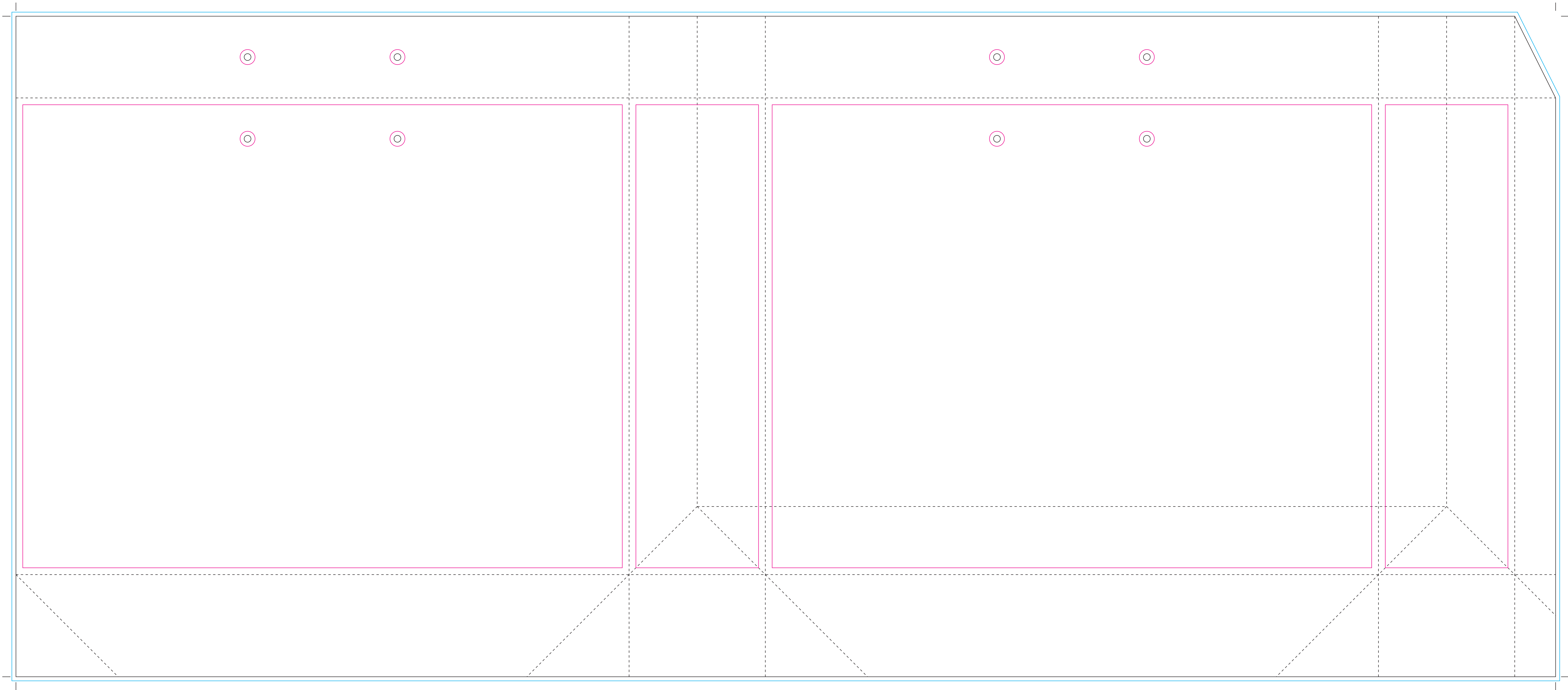
Paper Carrier bag - Type A Overall Size: 1130mm x 485mm — Cut --- Fold — Bleed — Text/Image Quiet Border (Text and images not running to bleed should be within this area)
